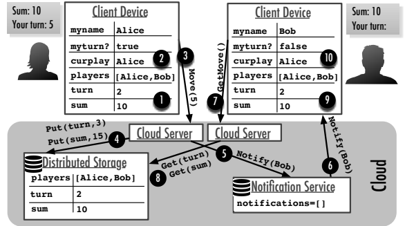
Figure 1: The 100 game. Each box is a separate address space. players, turn and sum are shared across address spaces and the storage system; myturn? and curplay are derived from shared data. When shared values change, the app manually updates distributed storage, other processes with the shared data, and any data in those processes derived from shared data, as shown by the numbered steps needed to propagate Alice’s move to Bob.
