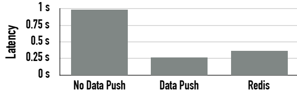
Figure 9: Latency comparison for 100 game rounds with data push notifications. Each round consist of 1 move by each of 2 players; latency is measured from 1 client. We implemented explicit data management and notifications using Redis and Diamond notifications with and without batched updates.
